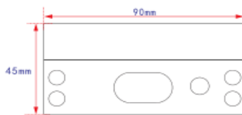
OEA-ES12-U Electric Bolt Lock U-Bracket
